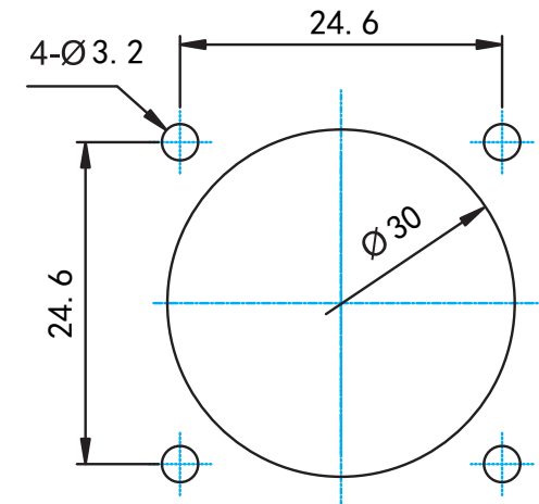
Cutout Dimension
